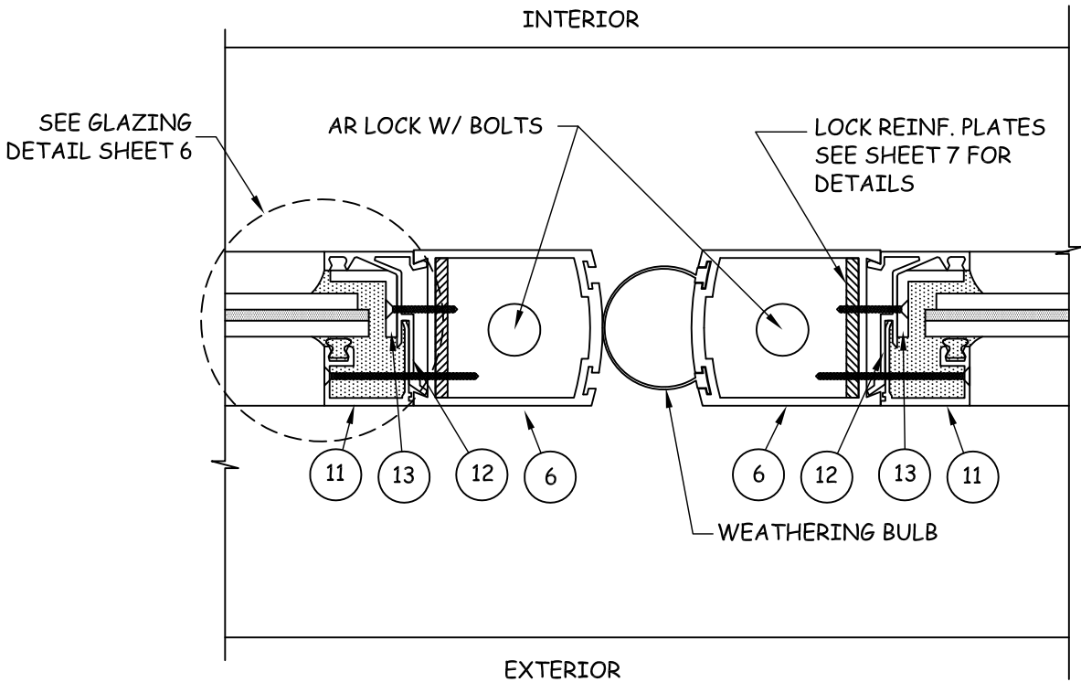
E 5 HORIZONTAL SECTION PANEL BUTT STILE
