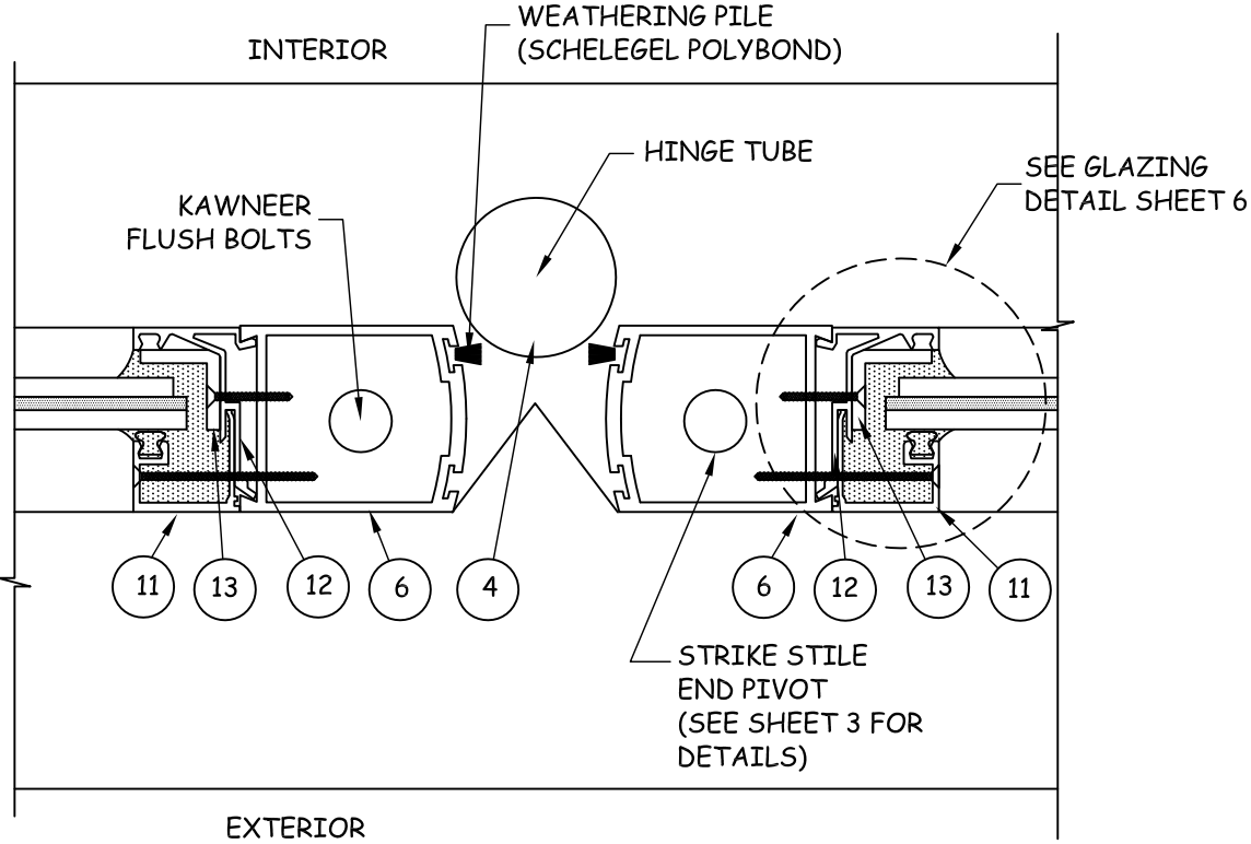
D 5 HORIZONTAL SECTION PANEL INTERLOCK
